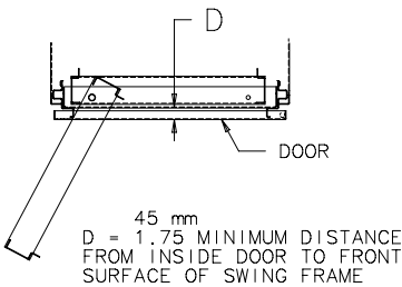
120° Mounting Position
