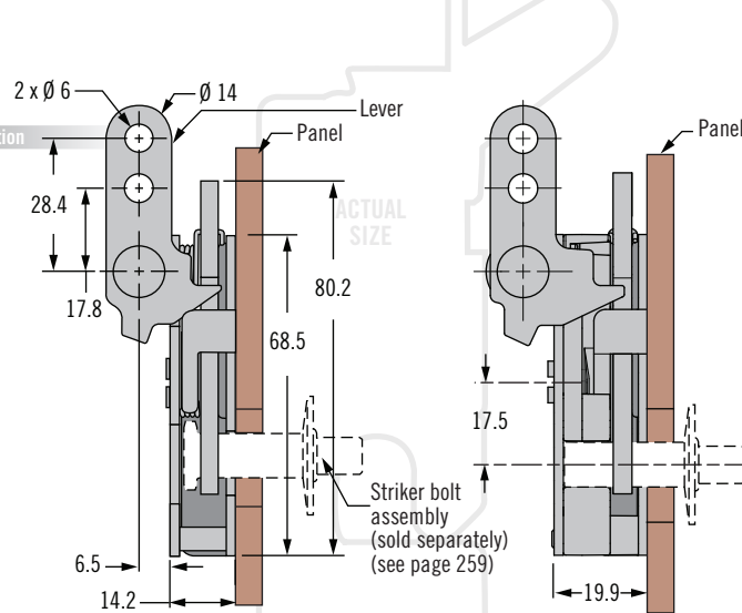
Integrated Bumper Version (dimensions same as standard version except as shown)
