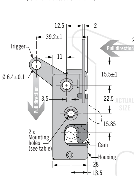
Single Stage - Dual Trigger - Bottom (left hand actuation shown)
