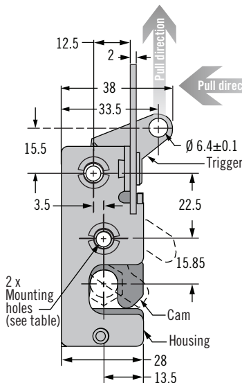
Single Stage - Dual Trigger - Top (left hand actuation shown)
