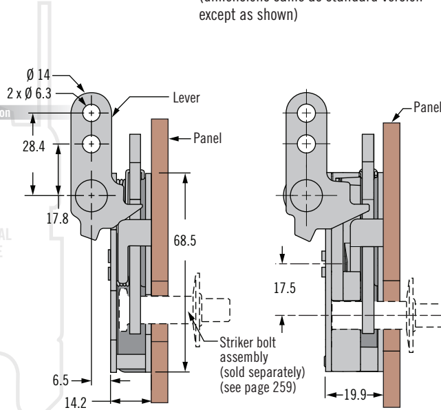
Integrated Bumper Version (dimensions same as standard version except as shown)
